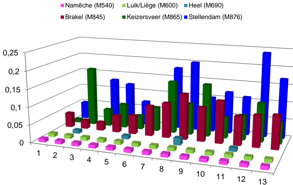
Figuur 12: Jopamidol in de Maas in 2011 [µg/l]
